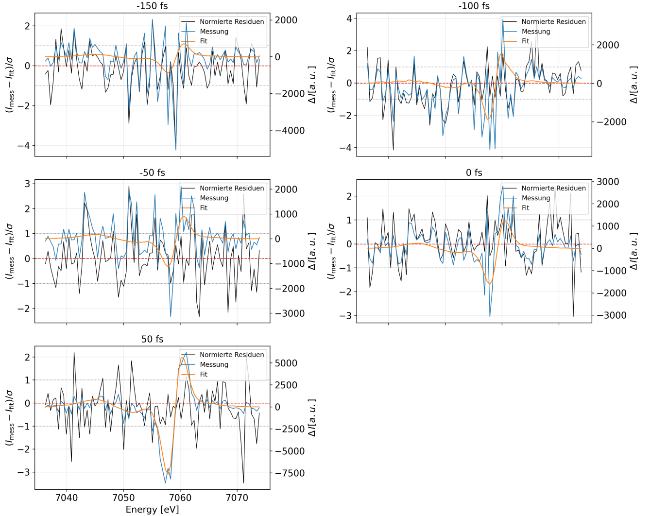
Figure 14: The normalised residuals together with the actual measurements and a fit over ... for time delays of \Delta t = \{-150 \text{ fs}, -100 \text{ fs}, -50 \text{ fs}, 0 \text{ fs}, 50 \text{ fs}\}
